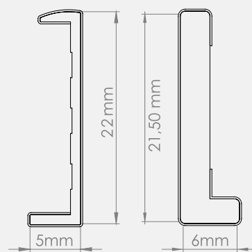
SIDE PROFILES (mm)
