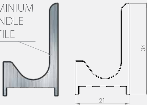
J HANDLE PROFILES (mm)
